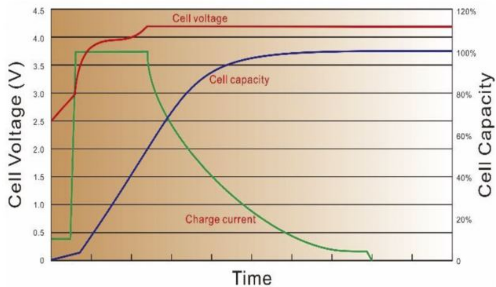
Charging Curve
