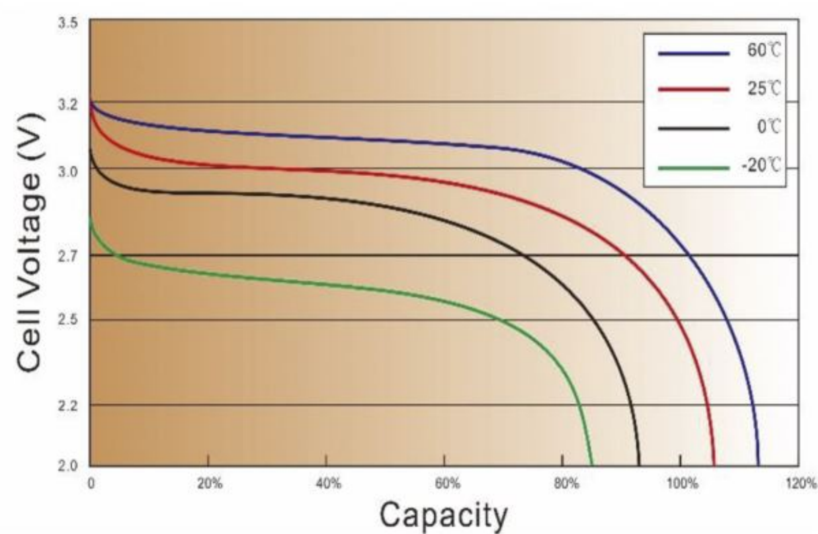
Discharge Curve At Different Temperature ( 1C )
