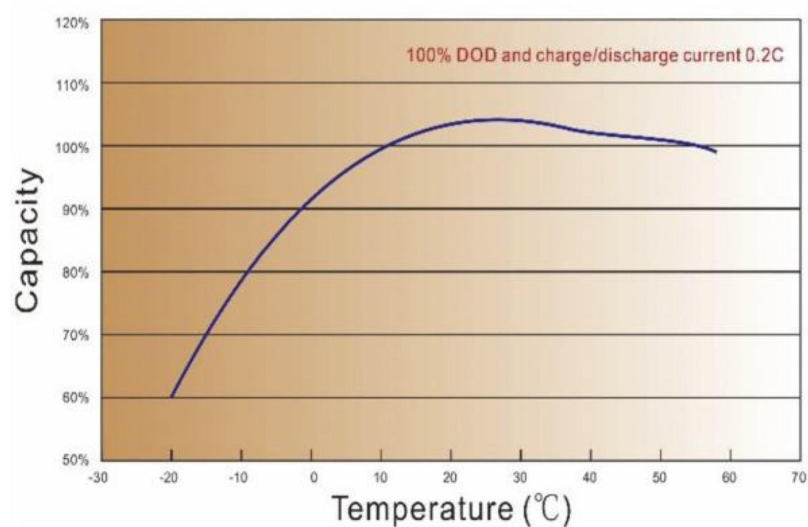
Temperature Effect In Relation To Battery Capacity
