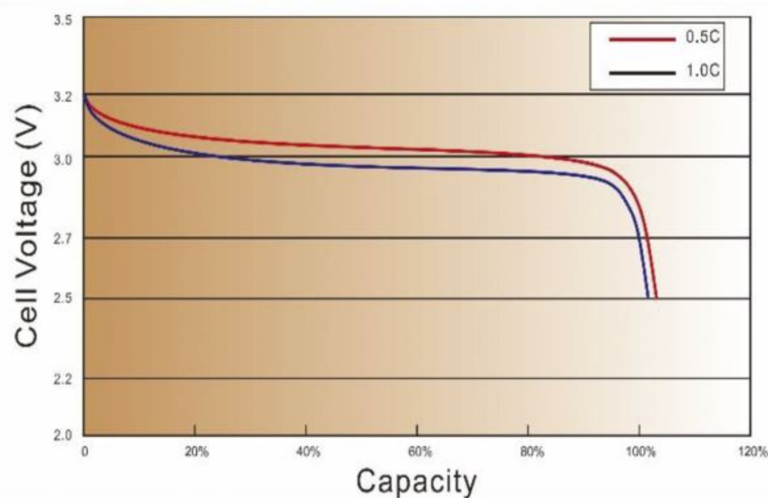
Discharge Capacity In Relation To Discharge Voltage
