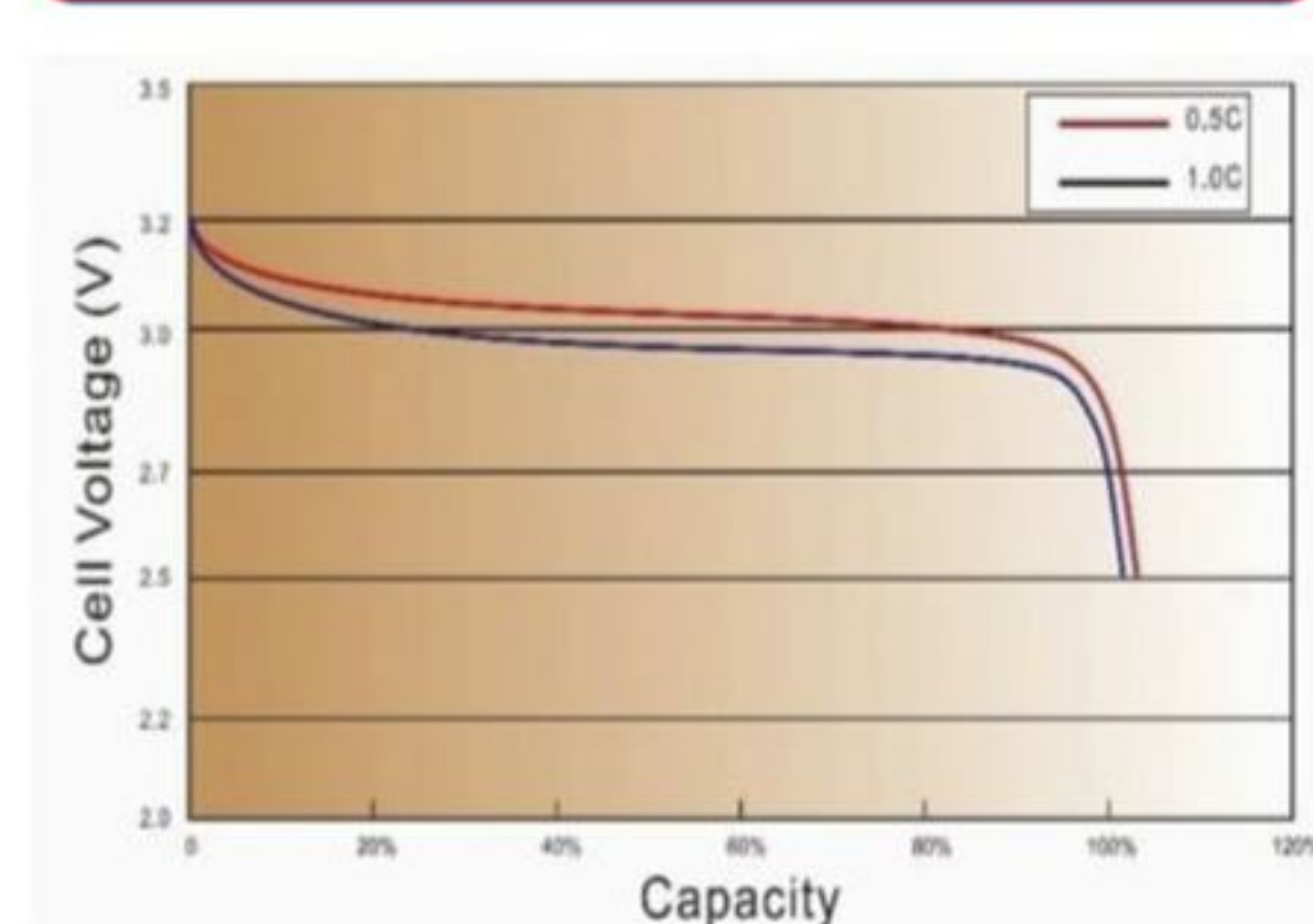
Discharge Capacity In Relation To Discharge Voltage
