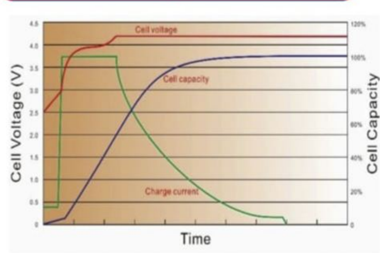
Charging Curve
