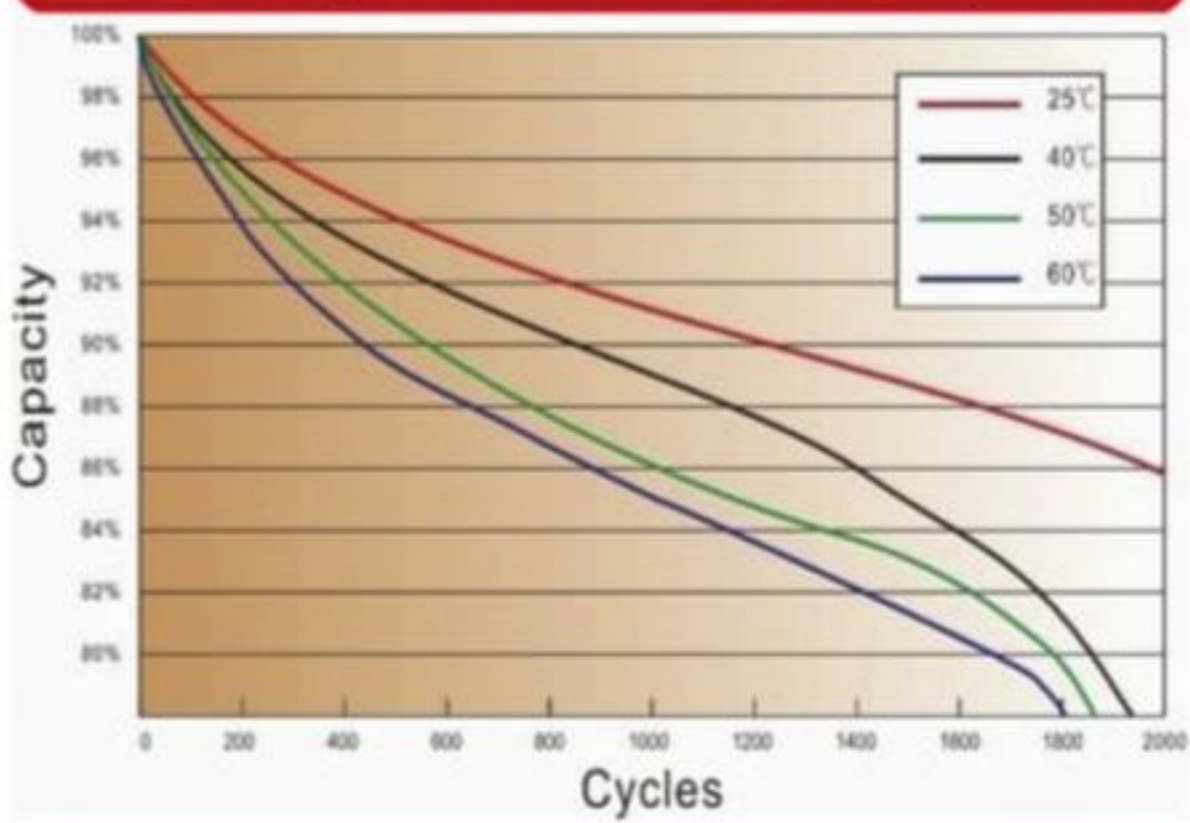
Temperature Effect In Relation To Battery Capacity
