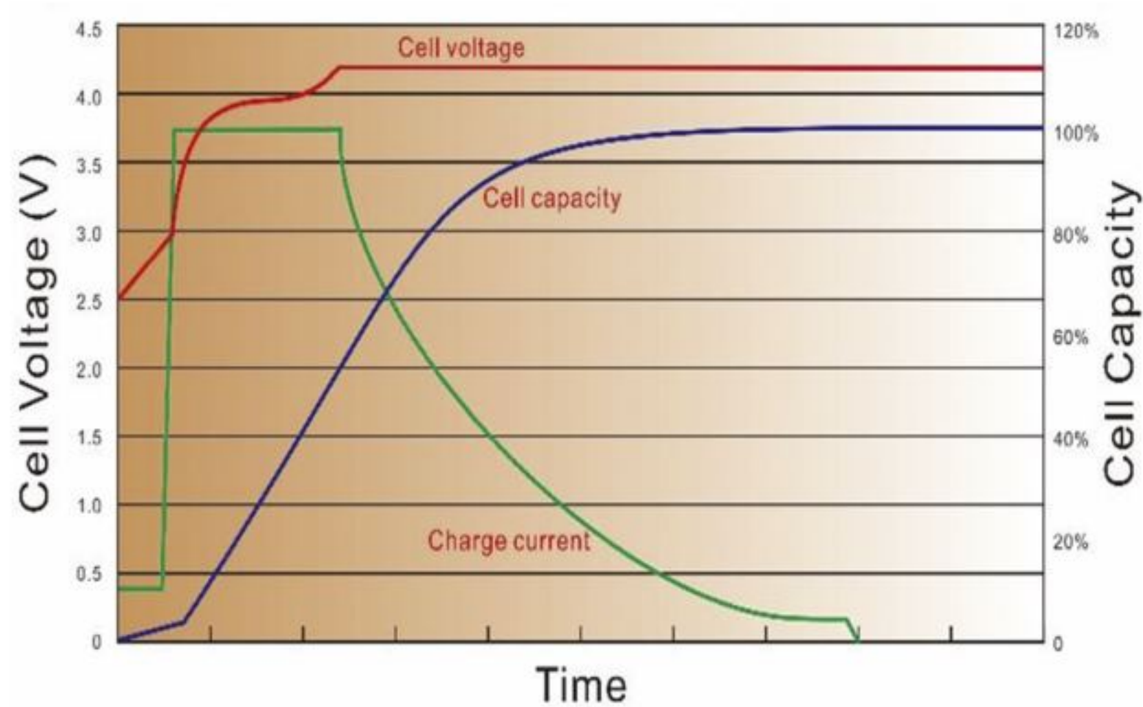
Charging Curve
