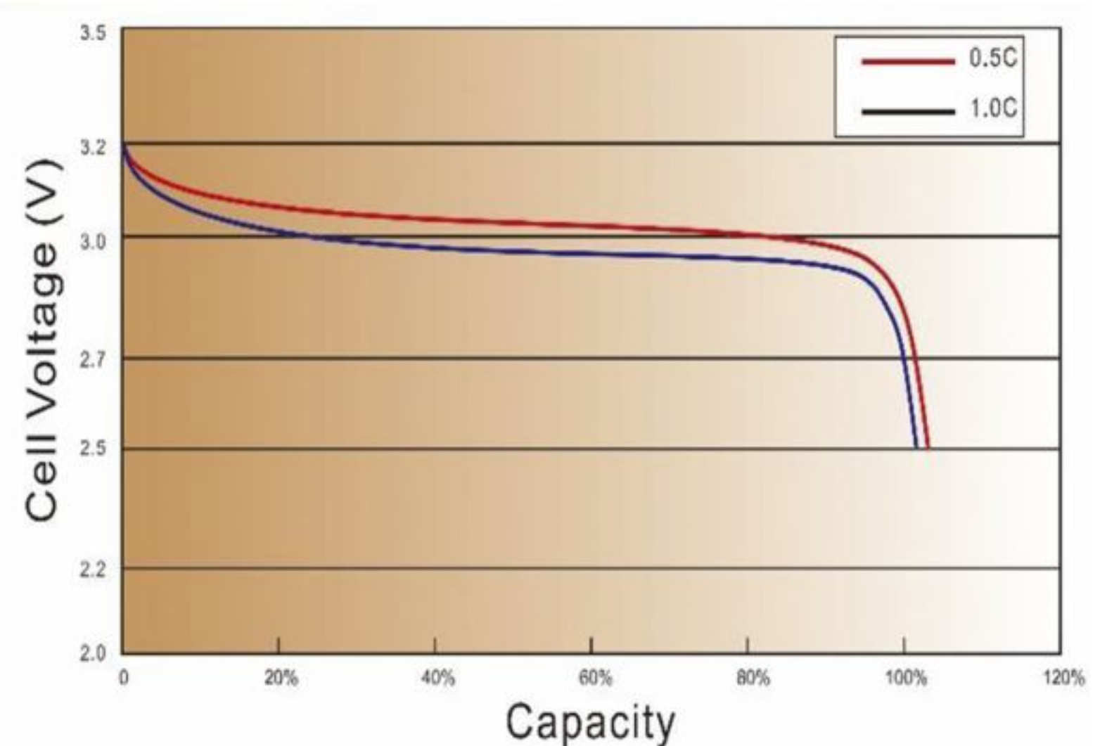
Discharge Capacity In Relation To Discharge Voltage
