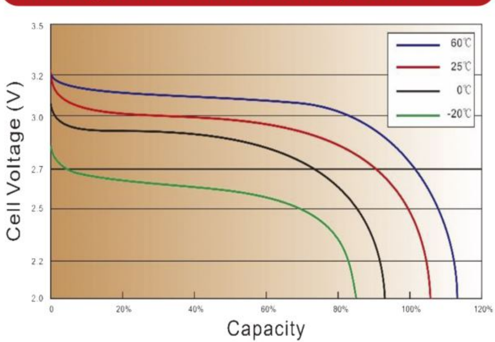
Discharge Curve At Different Temperature ( 1C )
