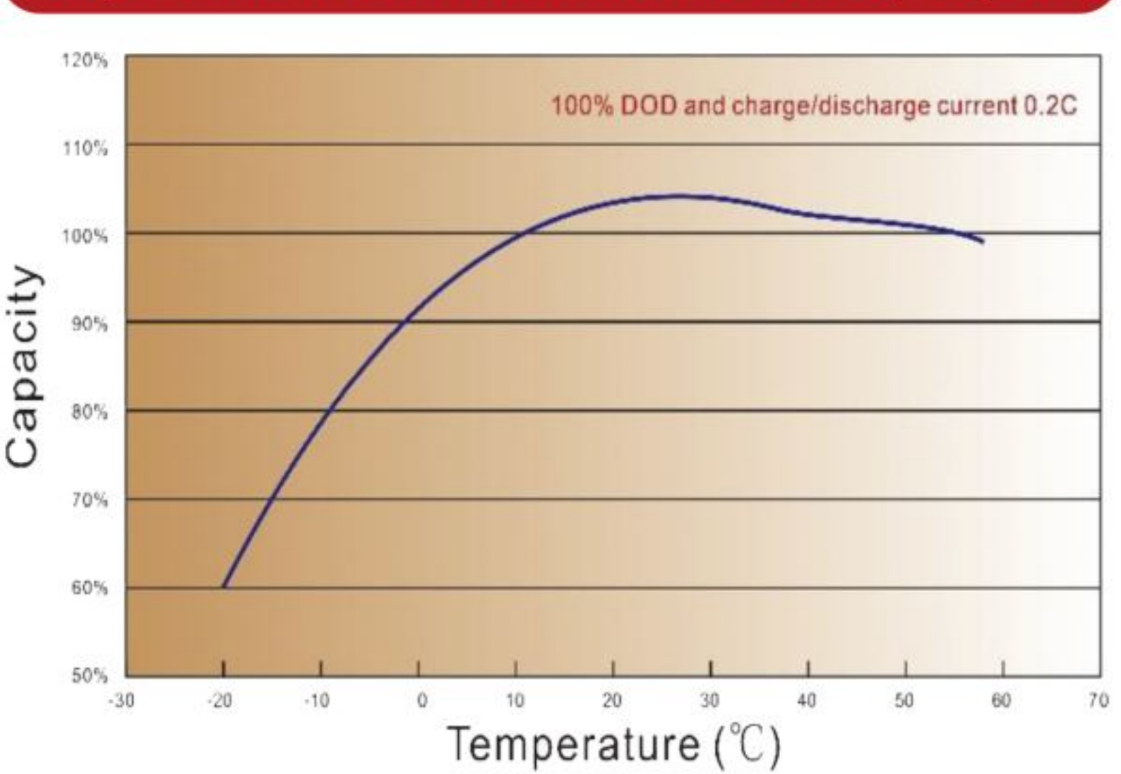
Temperature Effect In Relation To Battery Capacity
