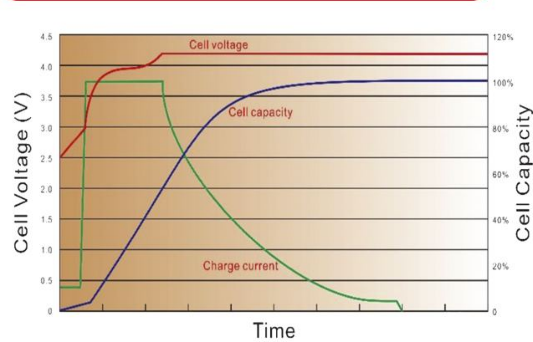
Charging Curve
