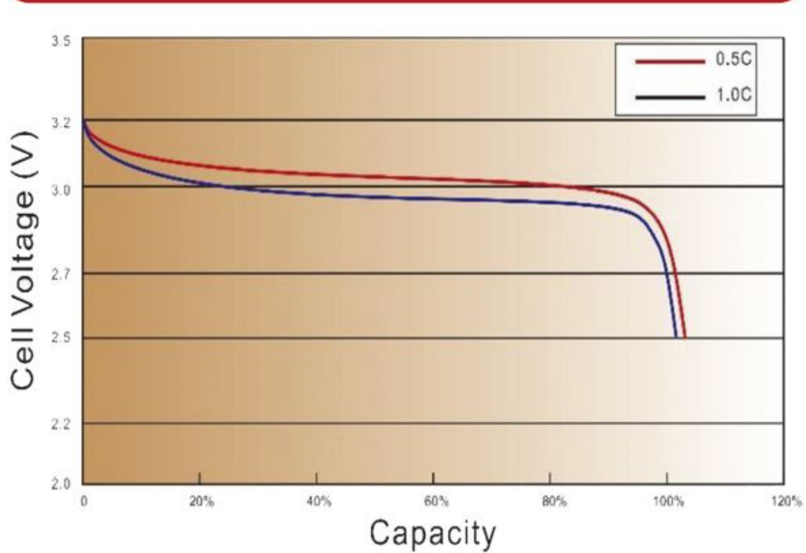
Discharge Capacity In Relation To Discharge Voltage
