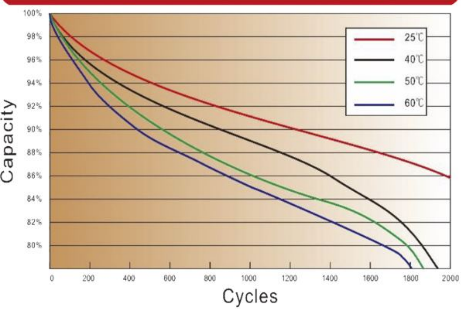
Temperature Effect In Relation To Battery Capacity
