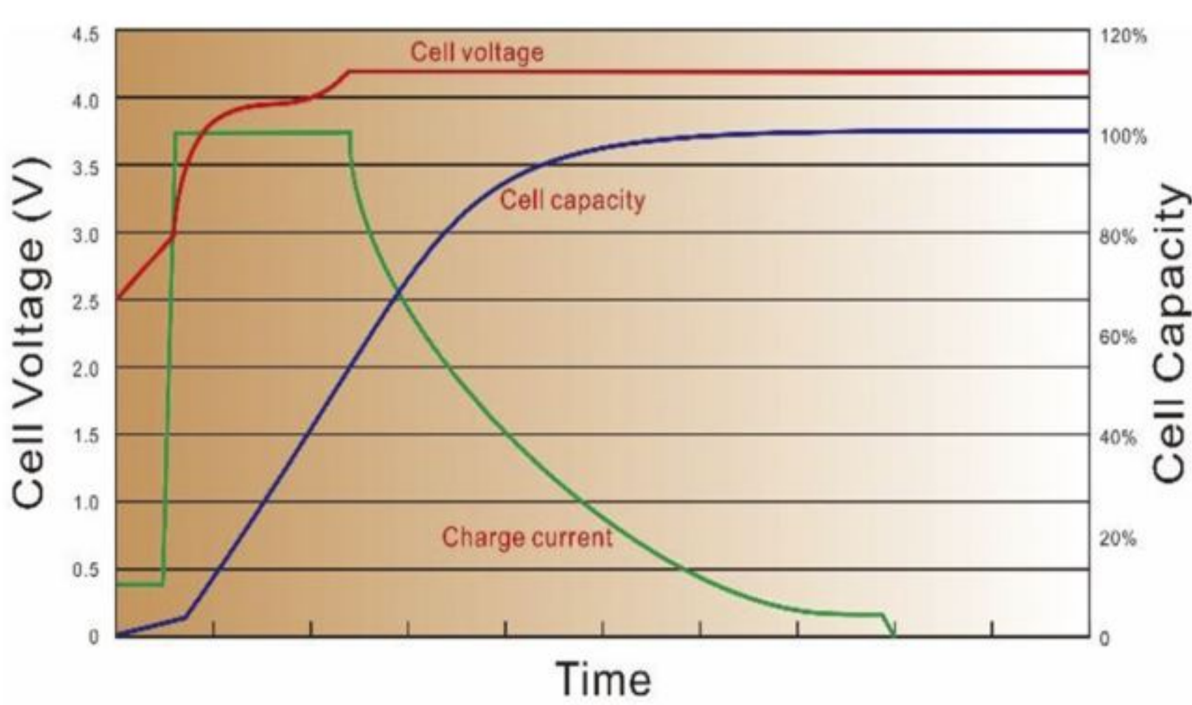
Charging Curve
